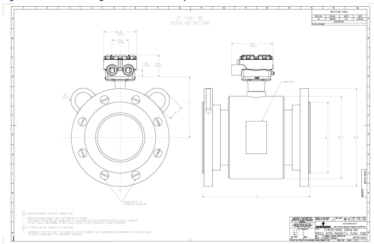
Figure 6: Model 8795 Magnetic Flow Tube R8 Option
