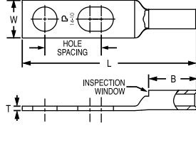
Figure 2 : Slotted, Straight
