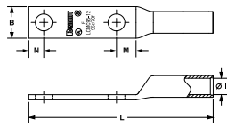
Figure 1. Two-Hole
