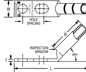
Figure 3 : Slotted, 45° Bent
